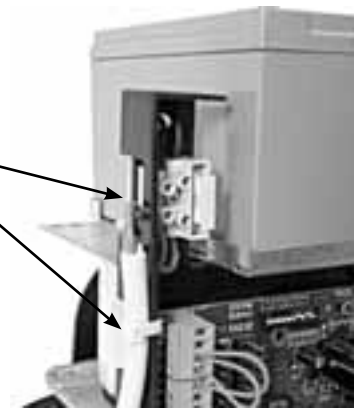
Wiring and fixing of power supply cable
