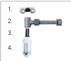
1. Anti-Theft Bracket 2. Adjustable Socket 3. Nylon Insert 4. Plate Gudgeon
